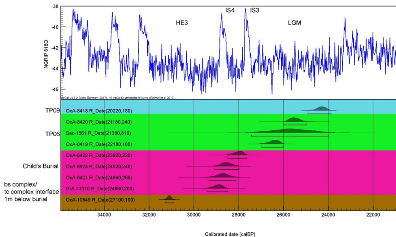
Fig. S1 - Figure S1. Relation of ^{14}\text{C} calibrated dates from Lagar Velho rockshelter with the NGRIP ^{18}\text{O} isotope curve. Radiocarbon ages have been calibrated using OxCal v. 4.3.2 (Bronk Ramsey, 2009a) and the Intcal13 curve (Reimer et al., 2013).
