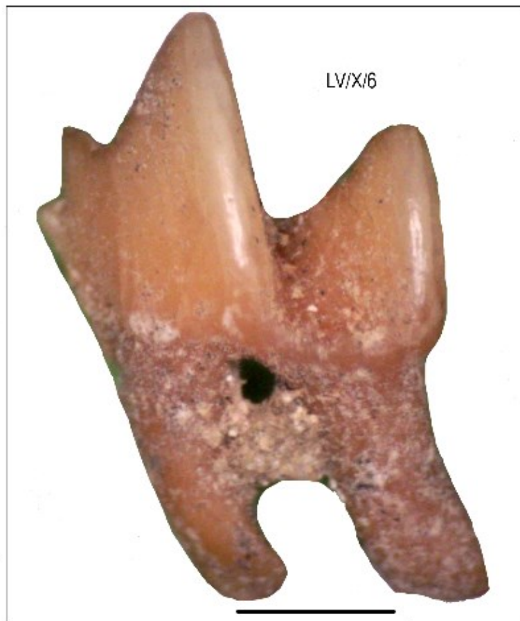
Figure S4. Left m2 Talpa cf. occidentalis . Scale 1 mm.
